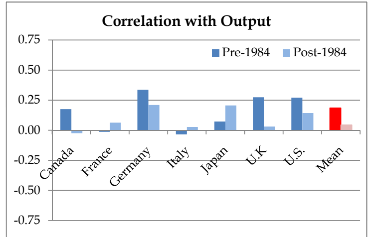
Chart 3. Cyclical Properties of Real Wages
