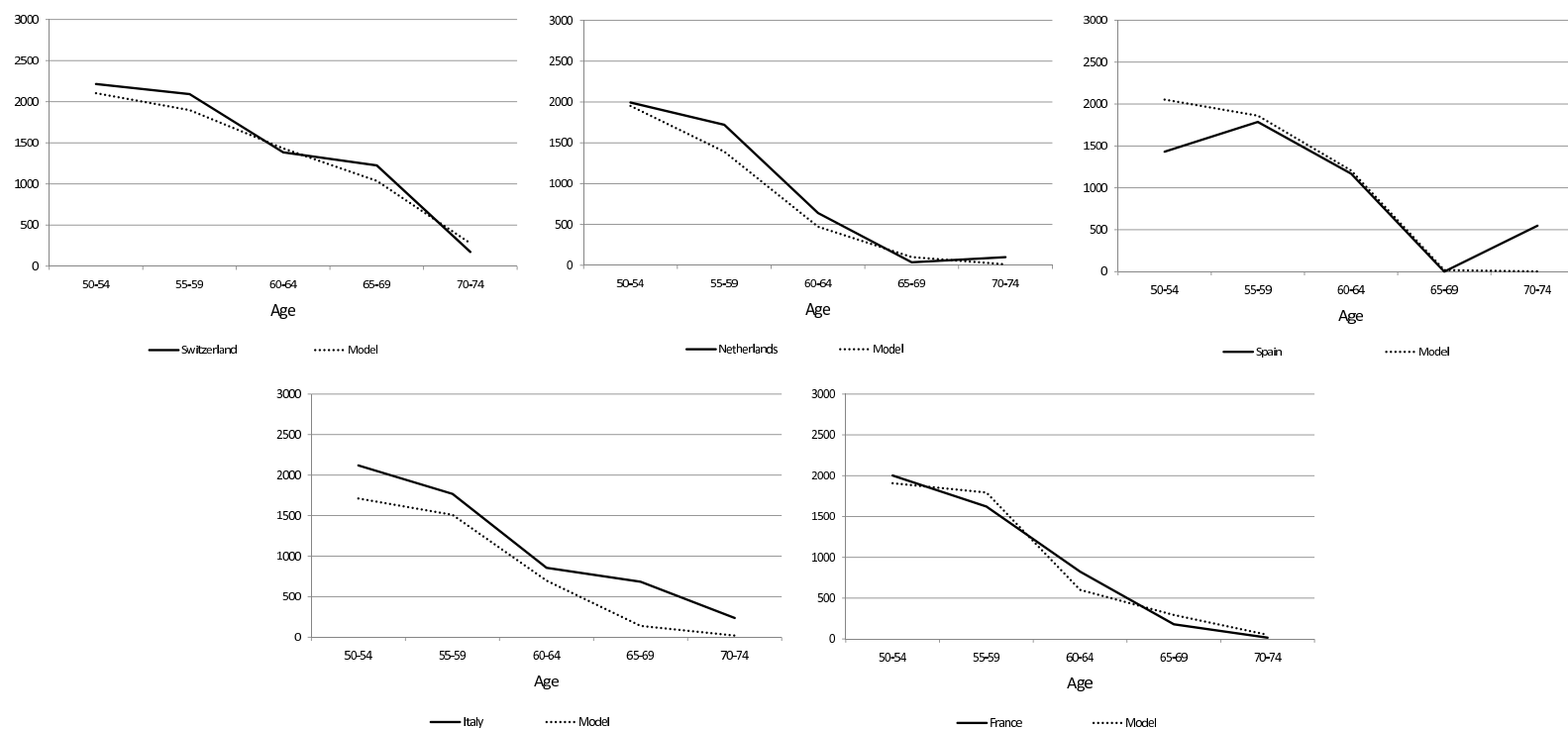
Figure A-7: Annual Hours Worked, College, Model vs. Data: Share 2004.
