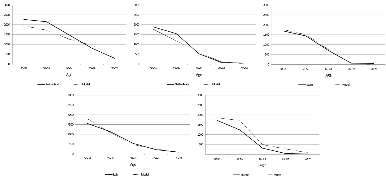
Figure A-5: Annual Hours Worked, All, Model vs. Data: Share 2004.
